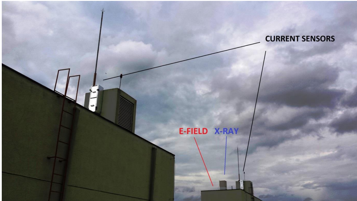
Figure 8. Location of the sensors on top of buildings P1 (left) and P2 (right).
