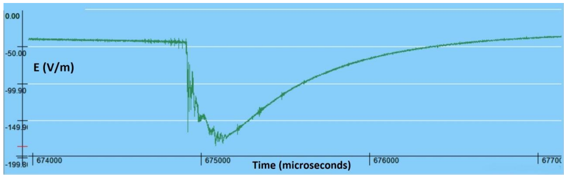
Figure 7. Electric field sensor and the signature of a lightning stroke.
