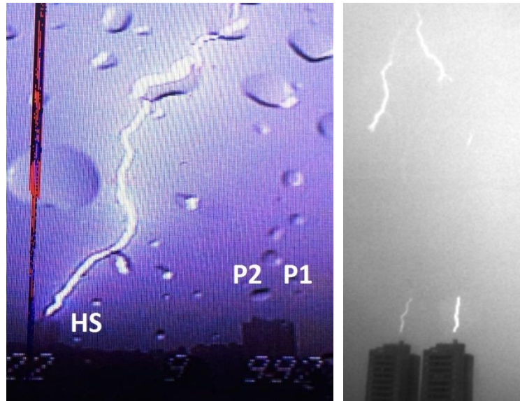
Figure 9. Negative cloud-to-ground flash striking building HS (image from standard video on left) and producing UUL from P1 and P2 on February 2nd, 2016 (image from high speed video on right).
