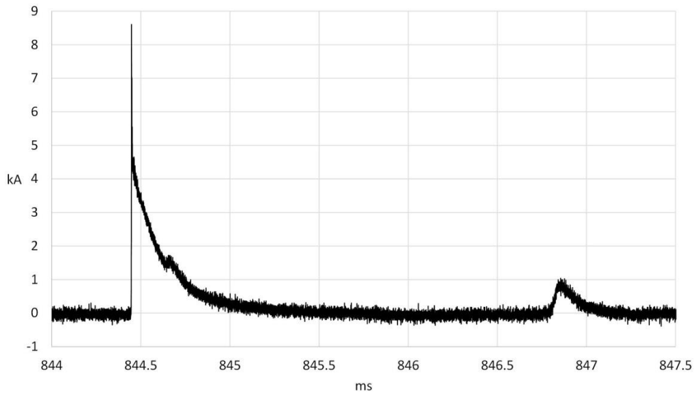
Figure 6. Current waveform of the second return stroke and following M-component the flash discharge that struck one of the lightning rods.
